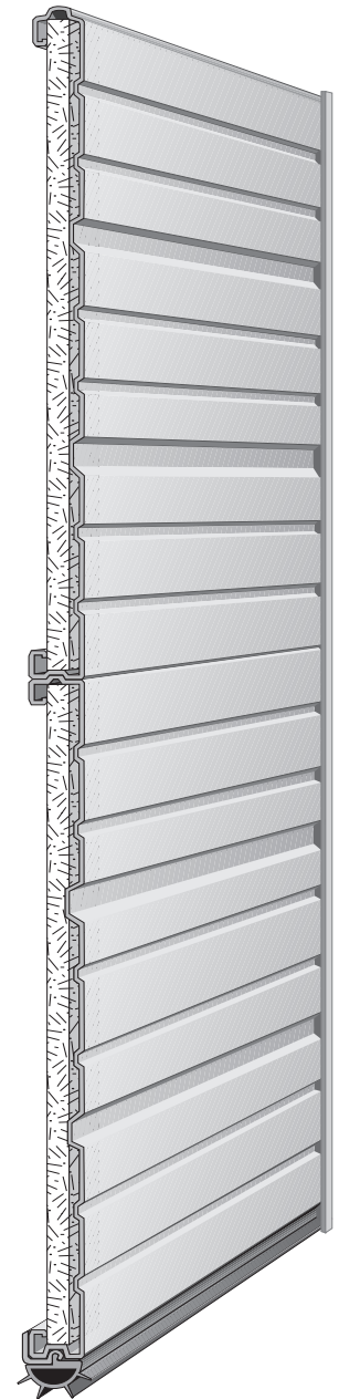
Bottom weatherstrip Full-length bottom PVC weatherstrip for superior airtight seal (Standard feature)
