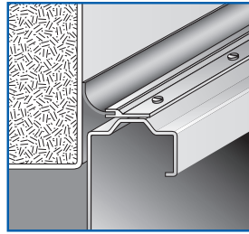
Top weatherstrip Vinyl header-seal at top
