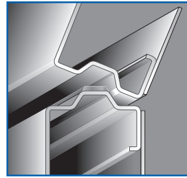
Joint weatherstrip Compressible foam gasket in tongue & groove joints
