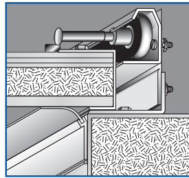
Jamb weatherstrip Flat aluminum with vinyl strip runs the full height of the door to seal against jambs.
