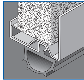
Bottom weatherstrip Full-length bottom PVC weatherstrip for superior airtight seal (Standard feature)
